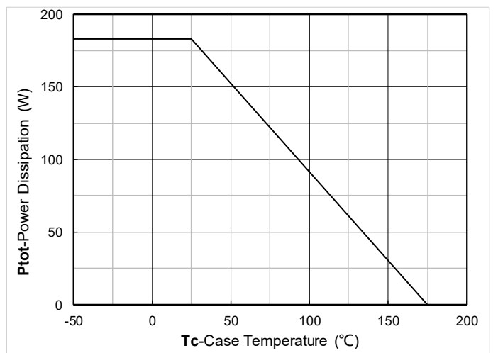
Figure 12. Power dissipation
